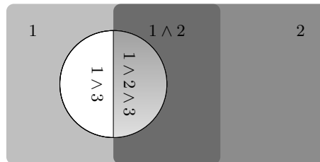
Fig. 2.4. The numbers reference the identifiers in Figure 2.1. 1 and 2 are overlapping rules and 3 is an exception to 1. In area 1 and 2 we conclude R_1 and R_2 respectively, while area 1 \wedge 3 leads to the conclusion R_3 . The conclusions in areas 1 \wedge 2 and 1 \wedge 2 \wedge 3 however is more involved, because R_1, R_2 respectively R_2, R_3 might be in conflict.
