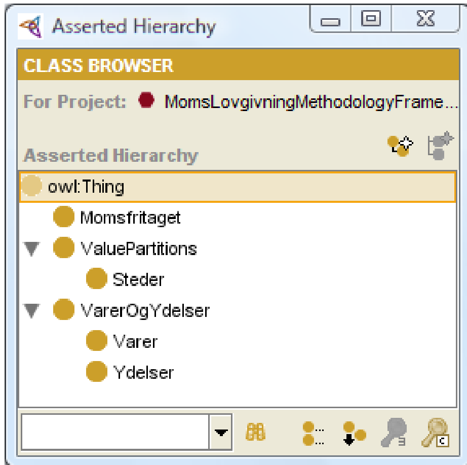
Fig. 2. Overall framework.
