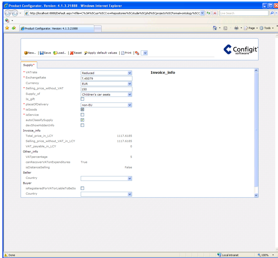
Fig. 3. Screen shot from the standard configurator where rule 11 takes precedence.
