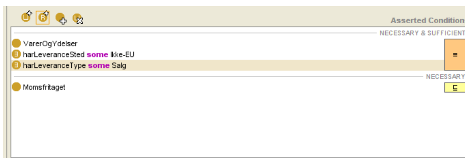
Fig. 4. Asserted Conditions of our model of the legal rule in Table 1.
